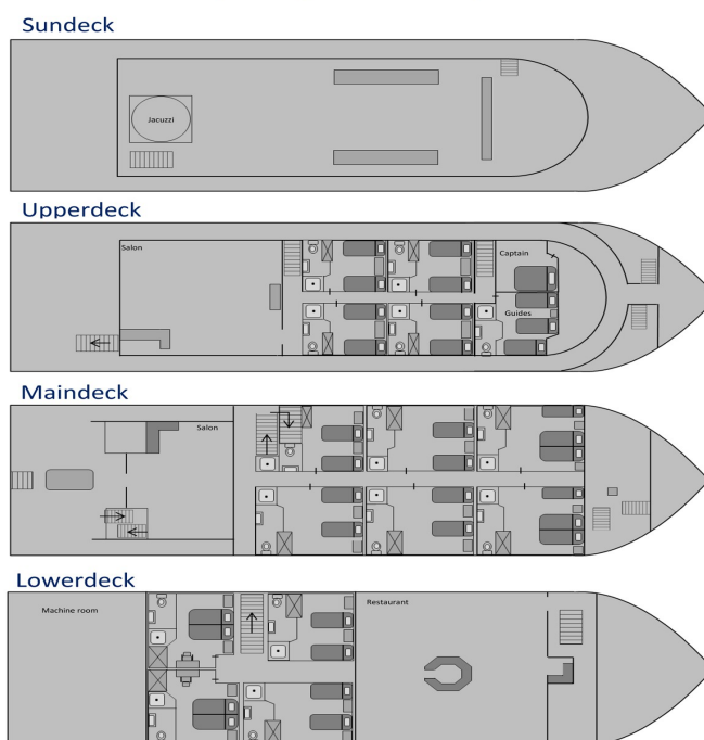
Deckplan M/Y Golden Dolphin IV
